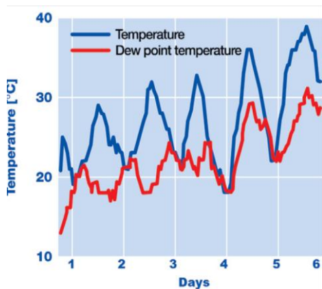
Transport without dew point control Condensation occurs when surface temperature and dew point temperature are equal.
