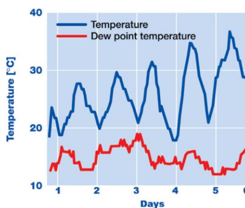
Transport with dew point control Dew point temperature is kept below surface temperature, preventing condensation and moisture damage.
